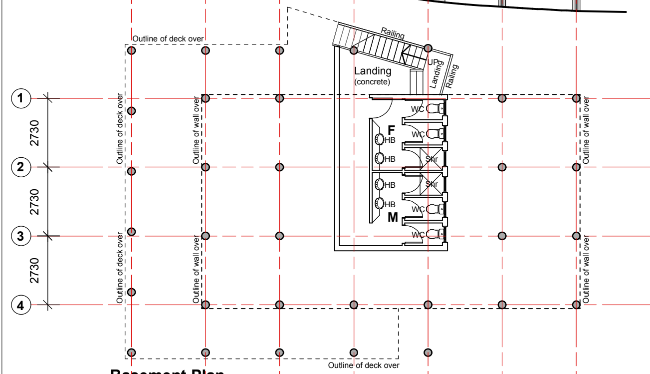
Basement Plan
